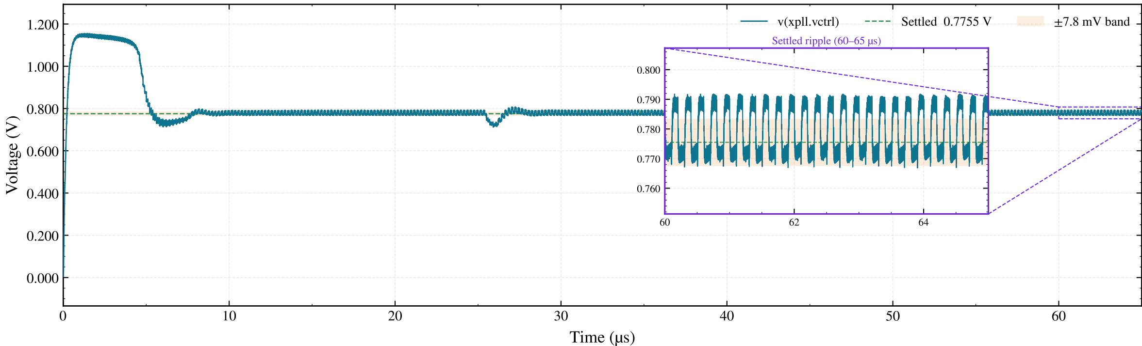
VCO Control Voltage — Lock-In Transient [0 \mu\text{s} – 65 \mu\text{s} ] SG13G2 130 nm BiCMOS | 2.4 GHz FPLL
