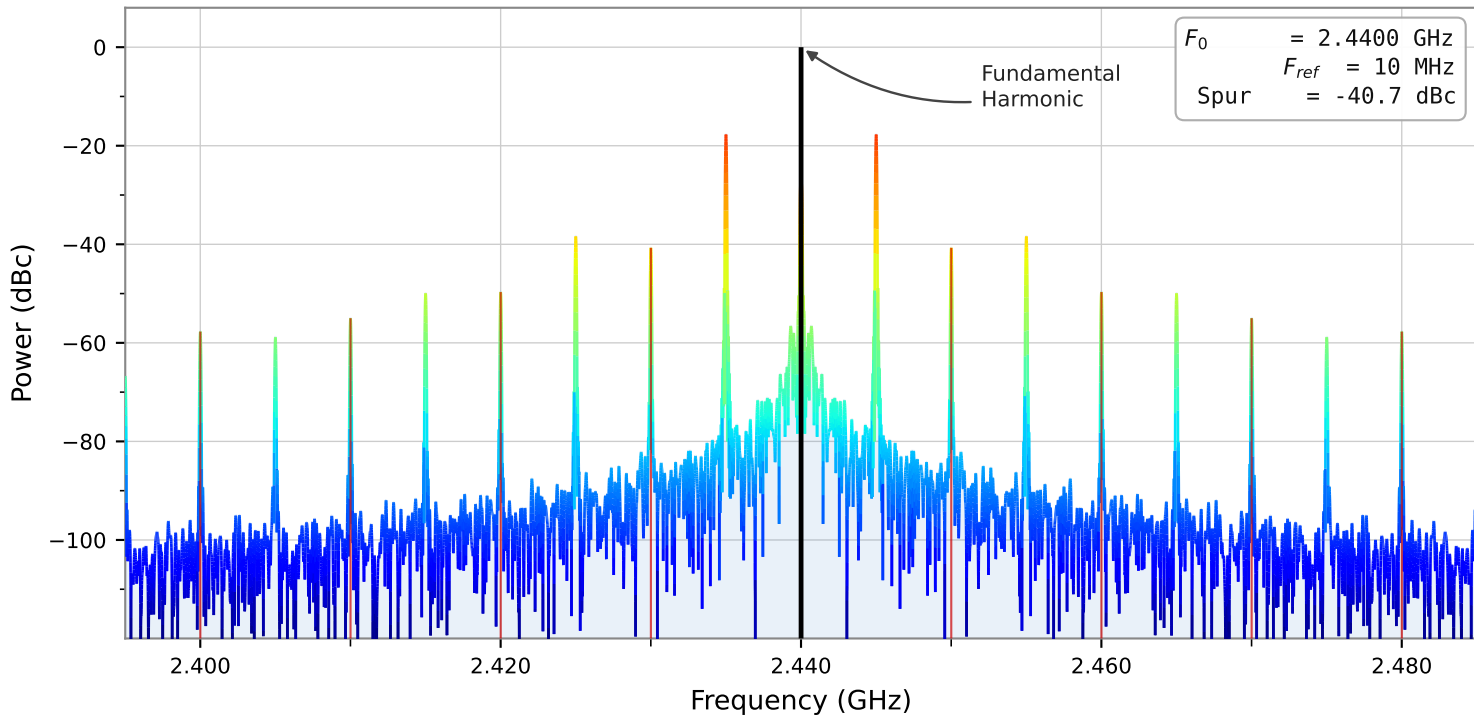
PLL Output Spectrum — Reference Spur: -40.7 dBc @ 10 MHz offset | f_0 = 2.4400 GHz
