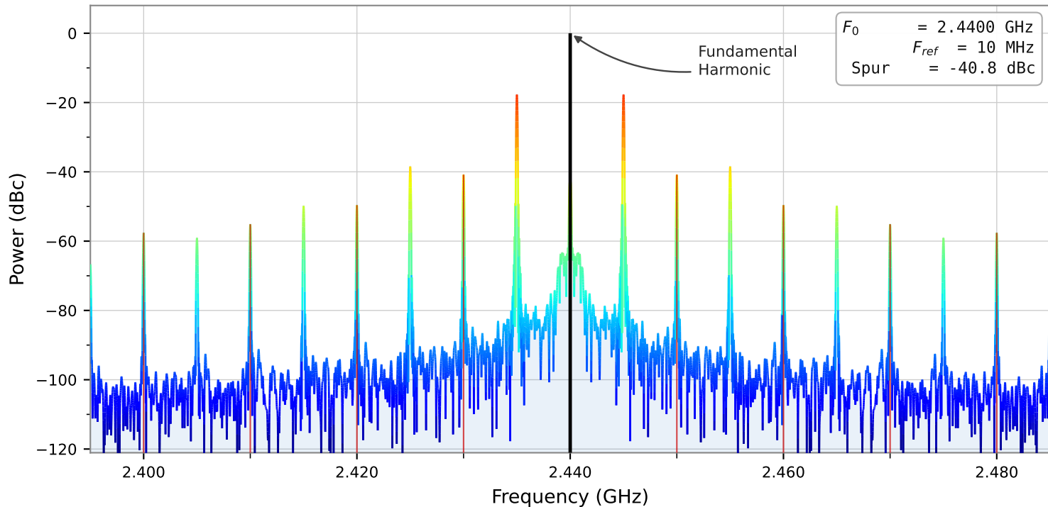
PLL Output Spectrum — Reference Spur: -40.8 dBc @ 10 MHz offset | f_0 = 2.4400 GHz
