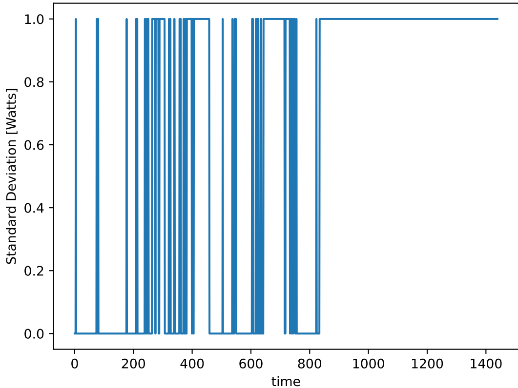
Cloudiness (Standard Deviation method)
