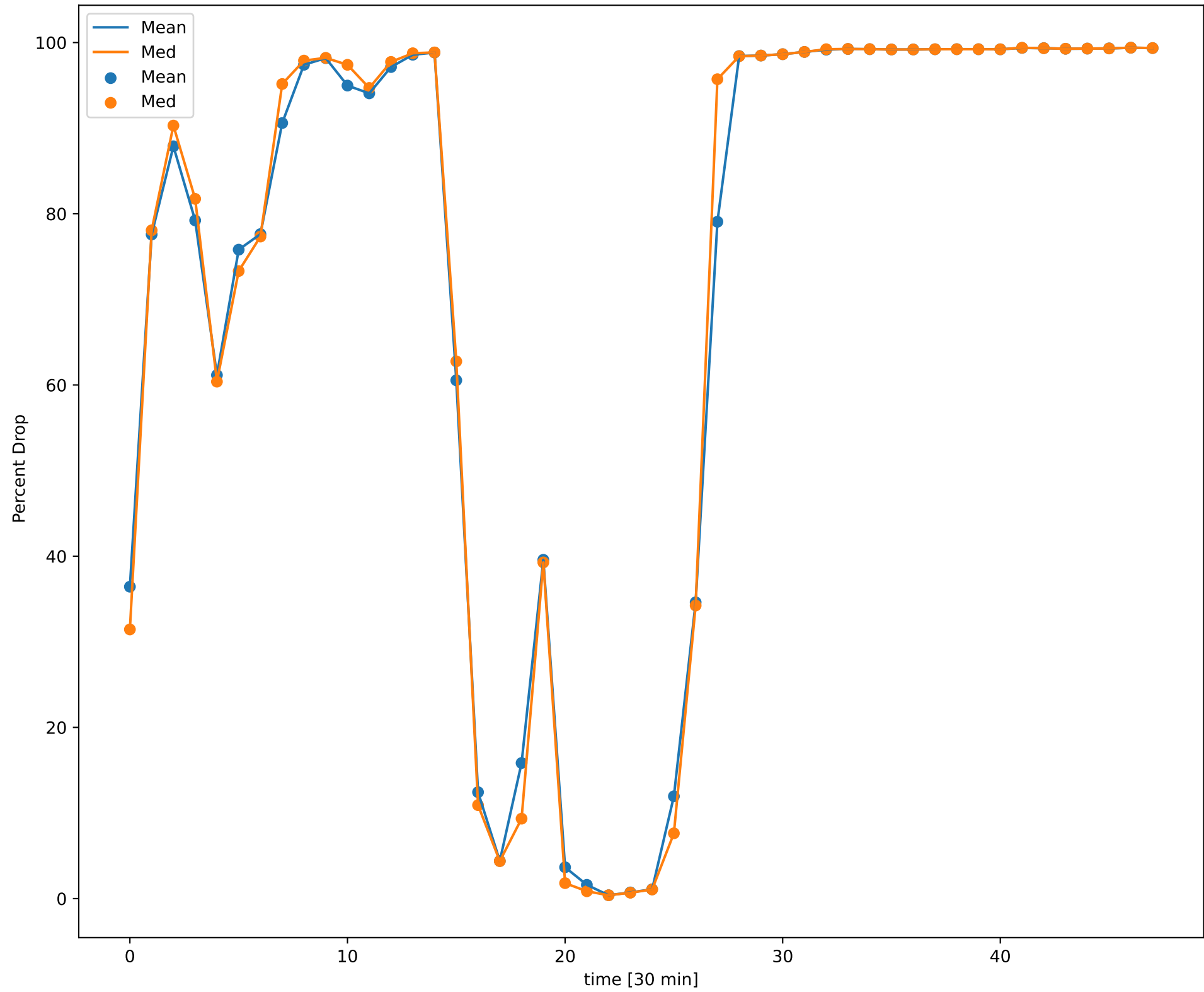
Half Hour Averages Percent Drop from Maximum Power 358, year 25
