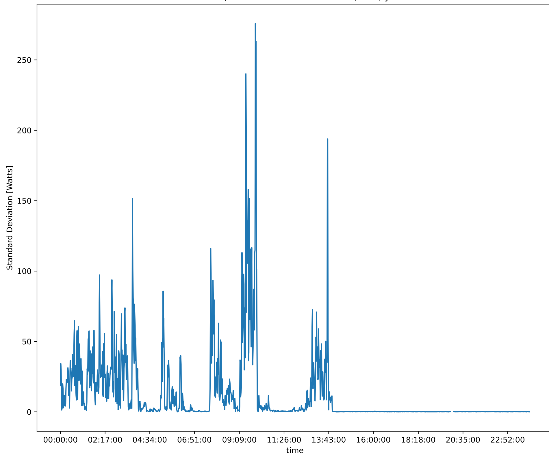
Cloudiness (Standard Deviation method) 358, year 25
