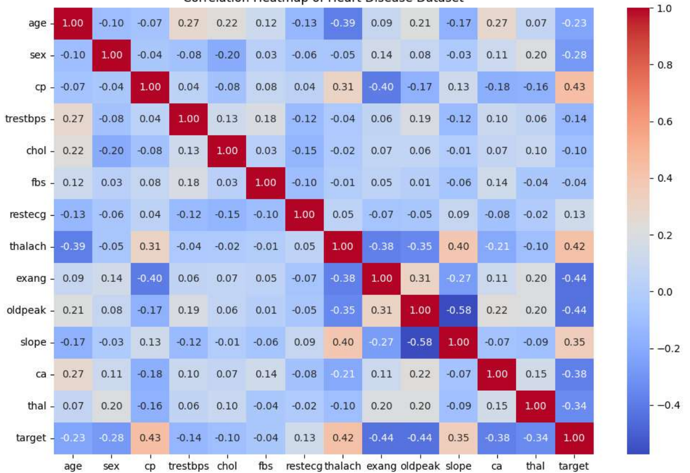
Correlation Heatmap of Heart Disease Dataset
