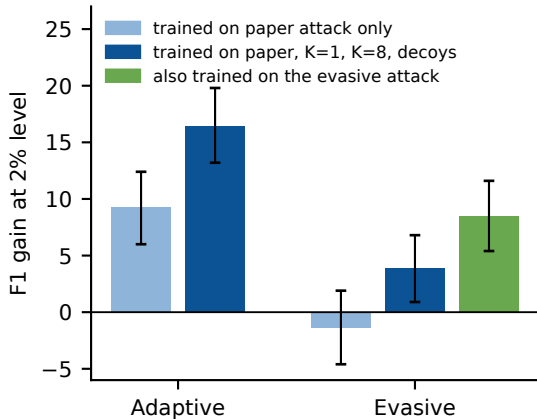
(b) coverage of the training attacks
