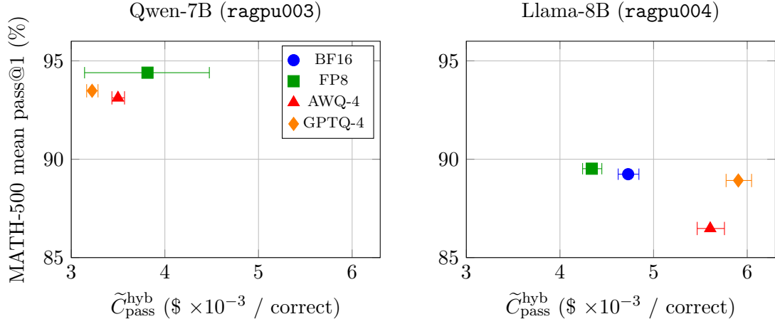
Figure 2: Confirmation Condition B aggregate hybrid Cost-of-Pass proxy versus campaign MATH-500 pass@1 ( \$ \times 10^{-3} ). Whiskers are 95% uncertainty intervals conditional on the observed timing repetitions and clustered accuracy bootstrap. Points are not joined. Panels are interpreted within model family; Qwen and Llama confirmation jobs ran on different hosts, so no pooled cross-host frontier is inferred. Within Qwen, Condition B nondominated points are FP8 and GPTQ-4; within Llama, FP8. Not a unique Pareto-efficient cell. Qwen FP8’s wide whisker is the five-rep wall-clock spread.
