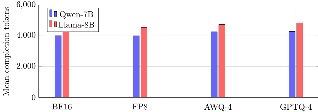
Figure 3: Full-grid mean MATH-500 completion tokens (ratio-of-means estimand). Bars are point estimates; clustered 95% intervals on paired token \Delta are in Table 5 and are not drawn on this axis.
