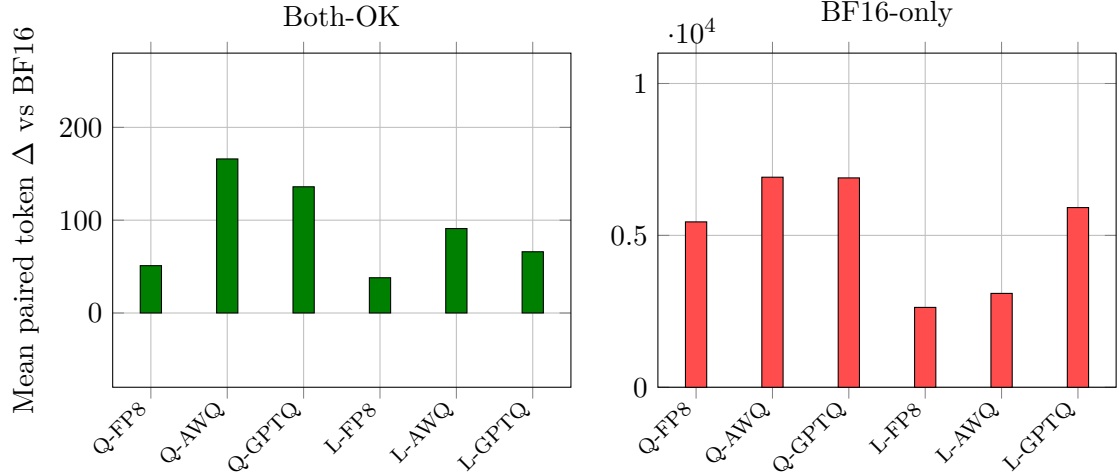
Figure 4: Paired token deltas by correctness, two panels so Both-OK is visible. Left: jointly-correct pairs (Qwen AWQ/GPTQ CIs exclude 0; FP8 and Llama CIs include 0; n in Table 5). Right: BF16-correct / quantized-wrong pairs. Clustered 95% CIs and n are in Table 5.
