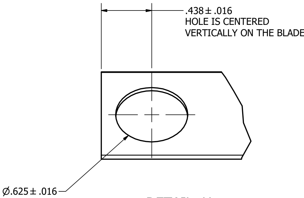
DETAIL H 2 PLACES SCALE 2 : 1
