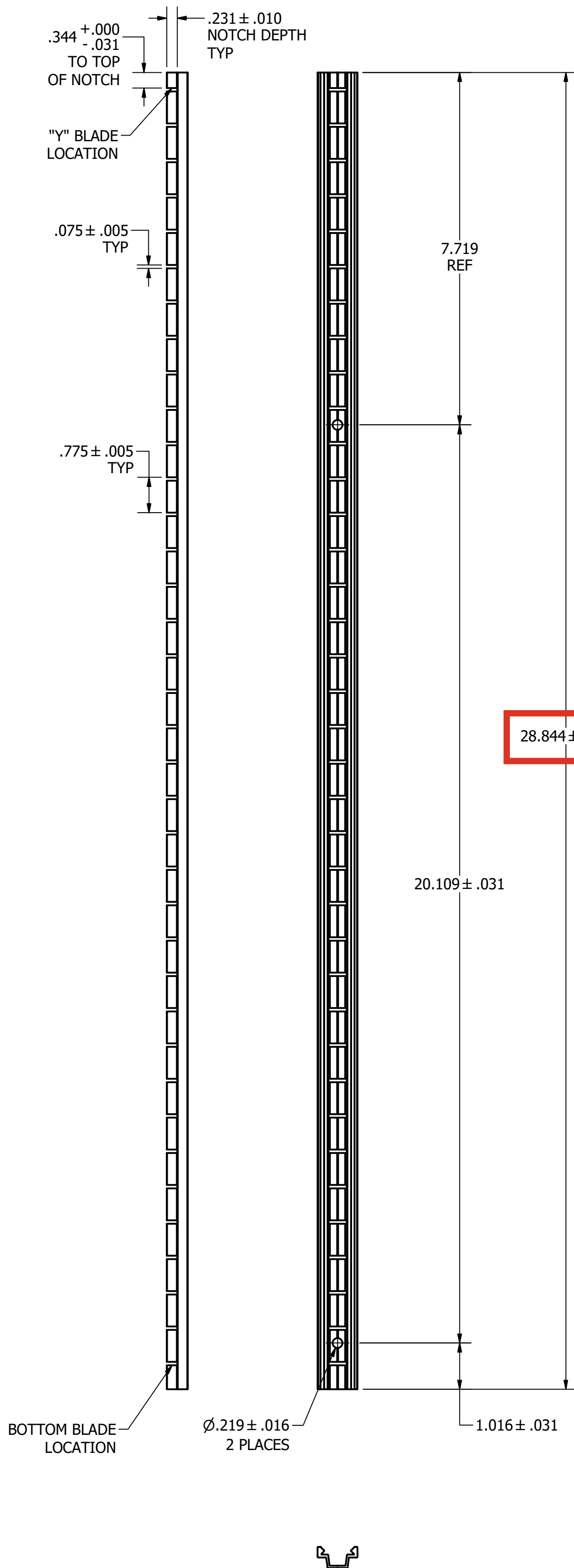
BRACE BAR - BOTTOM - MTG HOLE SCALE 1 / 2
