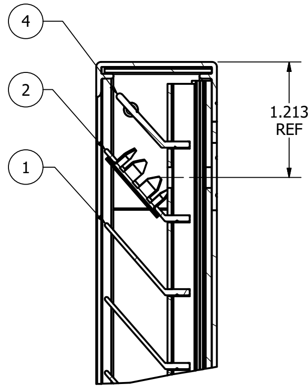
DETAIL E SCALE 1 : 1
