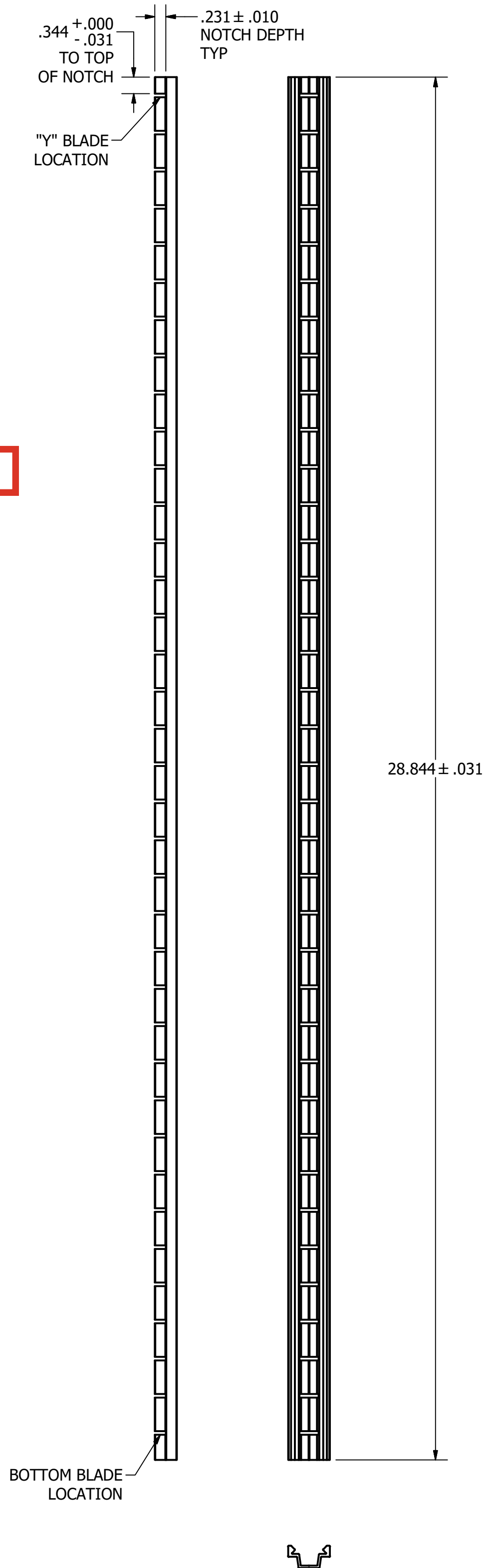
BRACE BAR - BOTTOM SCALE 1 / 2
