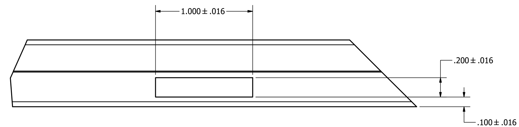
DETAIL K WEEP HOLES ON FRONT AND REAR FACE MUST BE ALIGNED SCALE 2 : 1
