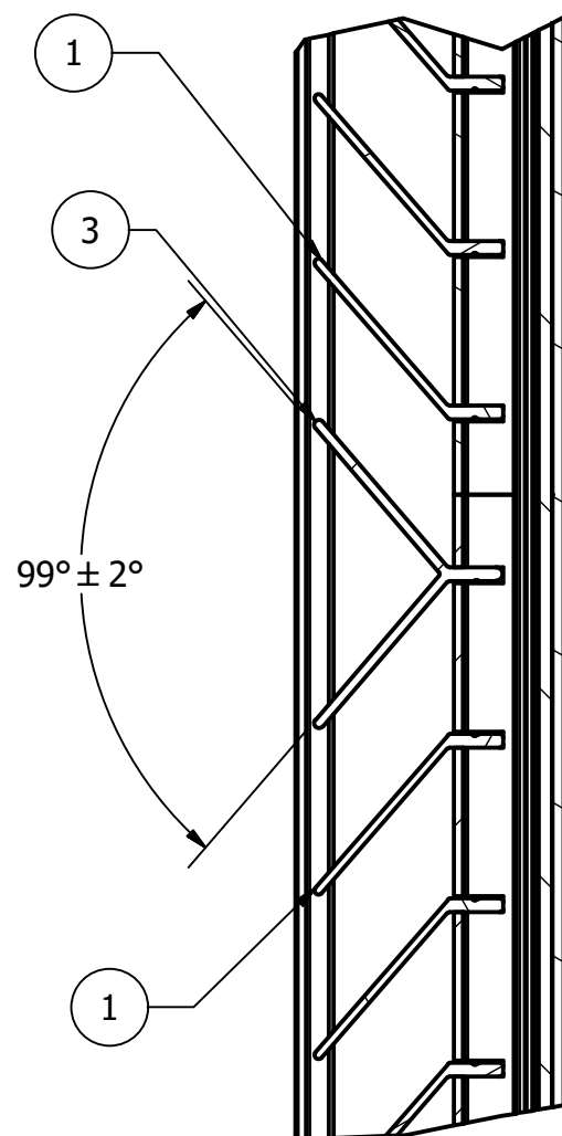
DETAIL D SCALE 1 : 1
