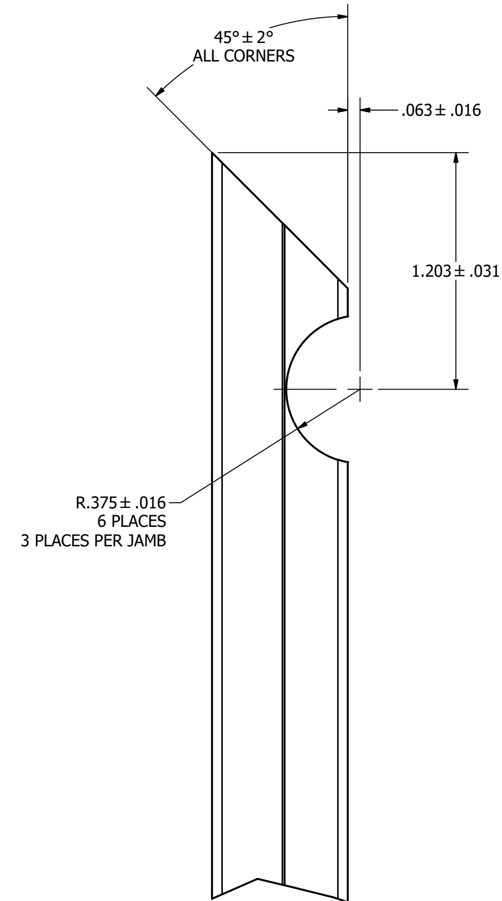
DETAIL J NOTCHES ON FRAME JAMB BACK LEG SCALE 2 : 1
