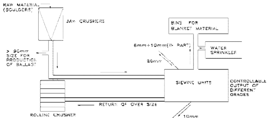
SCHEMATIC DIAGRAM OF MANUFACTURE OF BLANKET MATERIAL BY CRUSHERS
