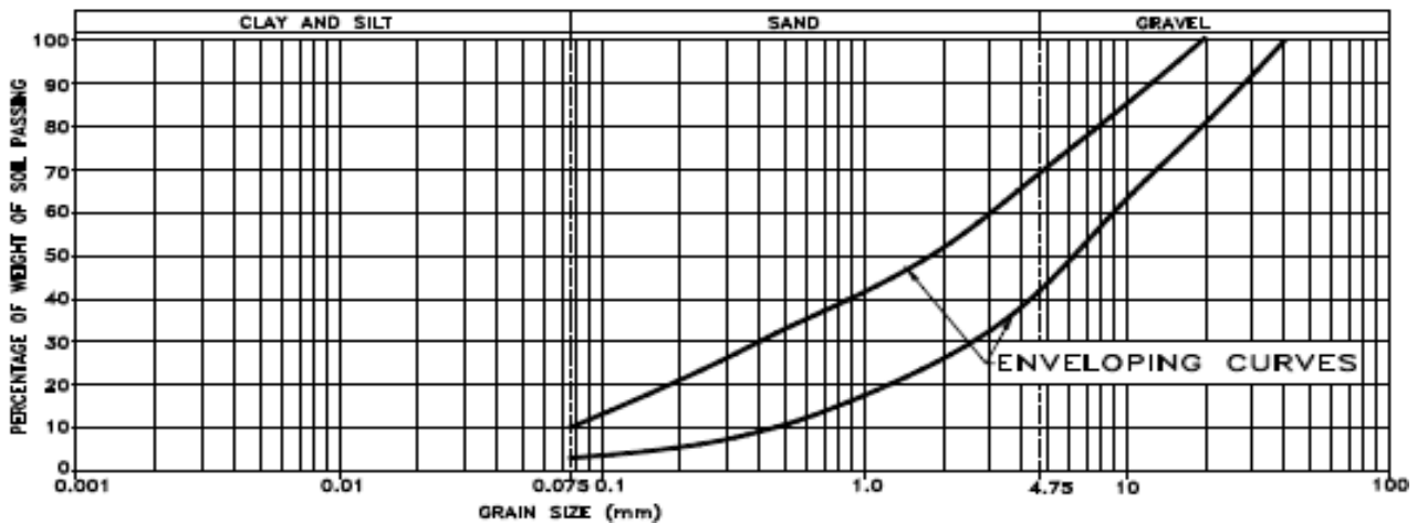
Fig. 9 : Enveloping Curves for Blanket Material:
