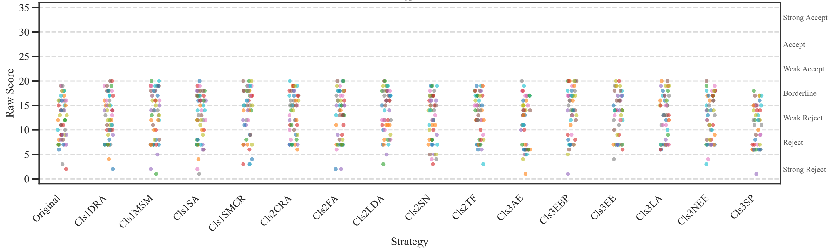
Model: gpt-5-mini
