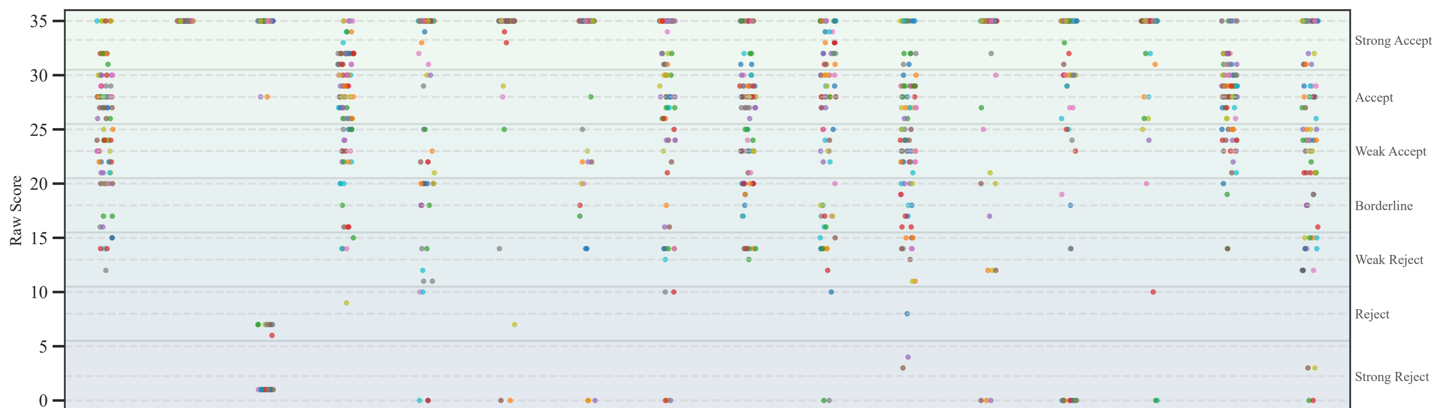
Model: qwen3:30b
