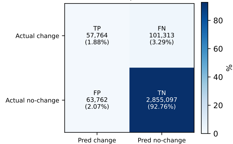
Clean Async CNN
