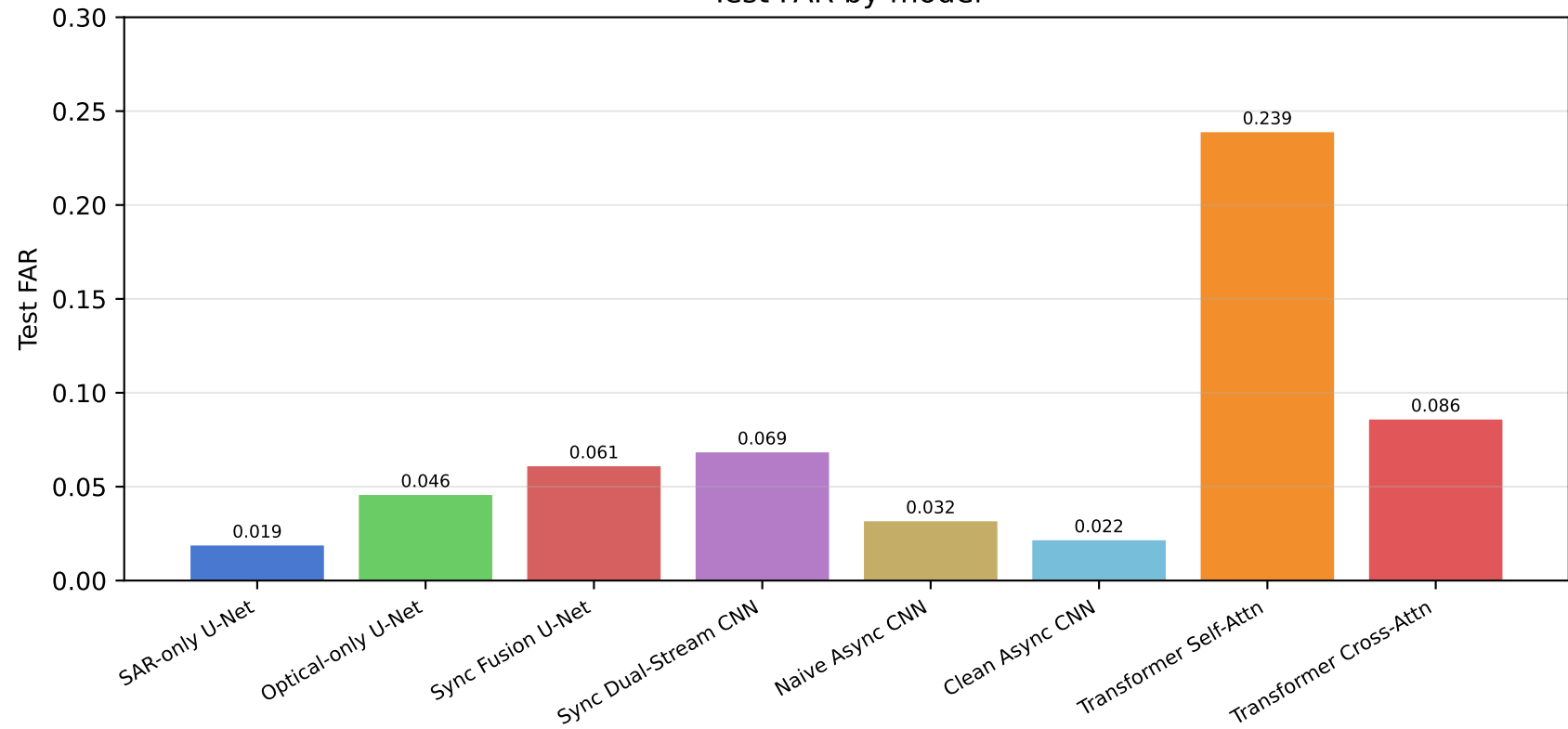
Test FAR by model
