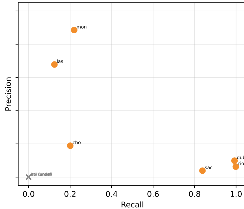
Transformer Self-Attn
