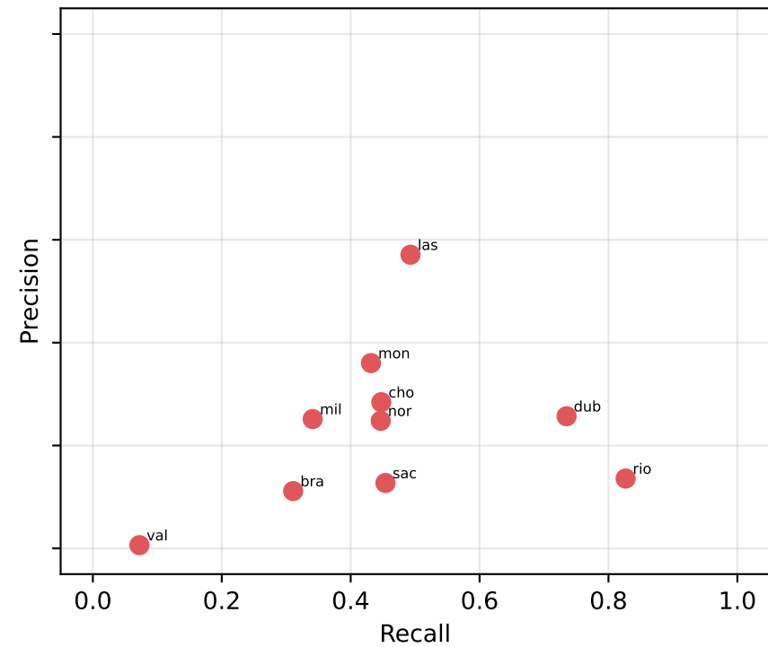
Transformer Cross-Attn
