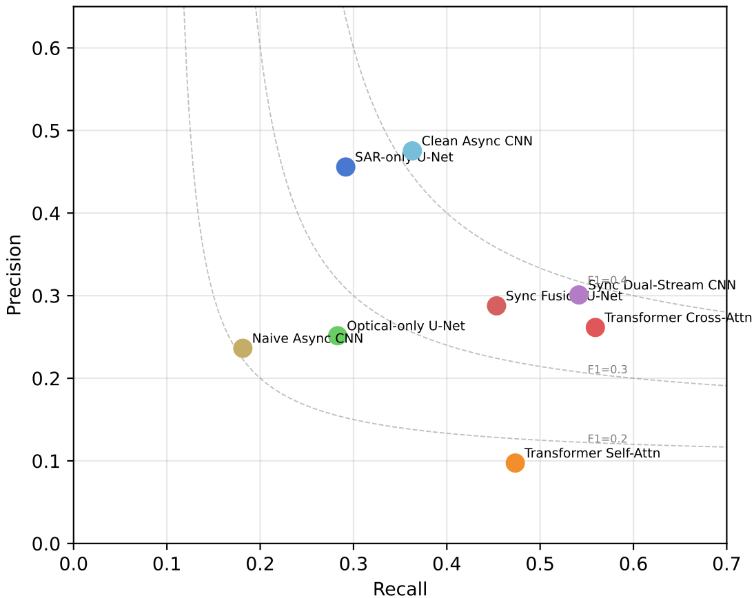
Precision vs Recall (test set)
