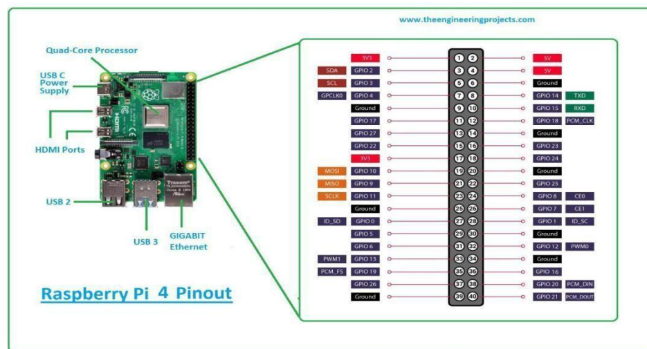
Fig : 3.2 Raspberry Pi 4B Board with Pinout
