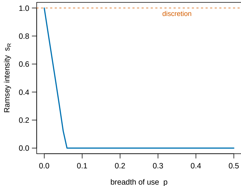
(b) optimal rule by breadth
