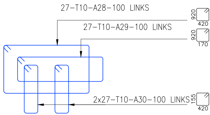
LINKS DETAILS SCALE 1:25
