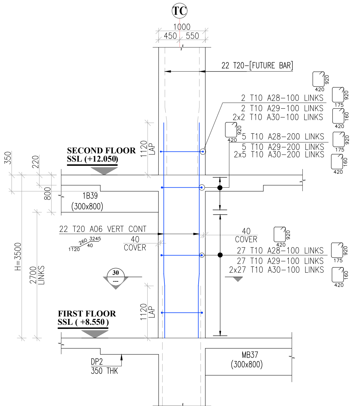
DETAIL-30A-C2 (500x1000) - 1 Nos. SCALE 1:50
