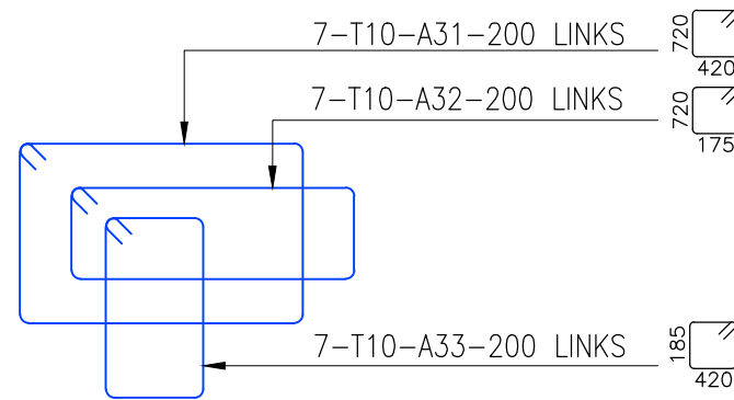
LINKS DETAILS SCALE 1:25
