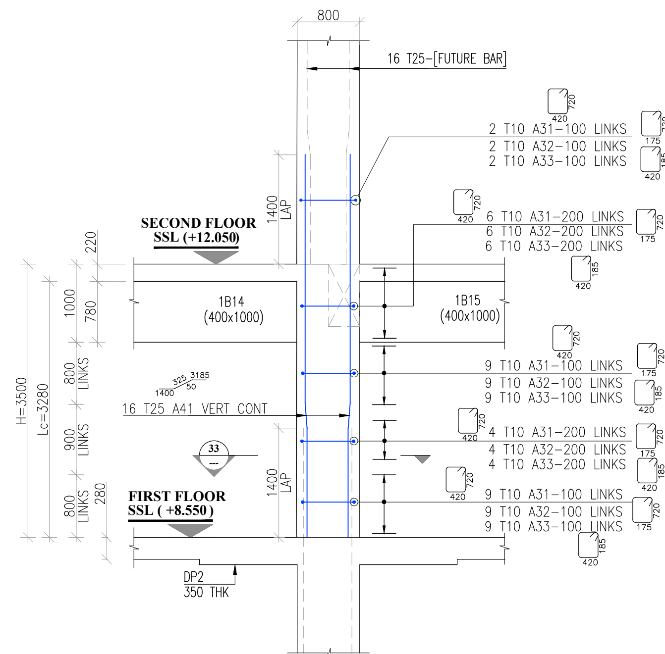
DETAIL-33A-C4 (800x500) - 1 Nos. SCALE 1:50
