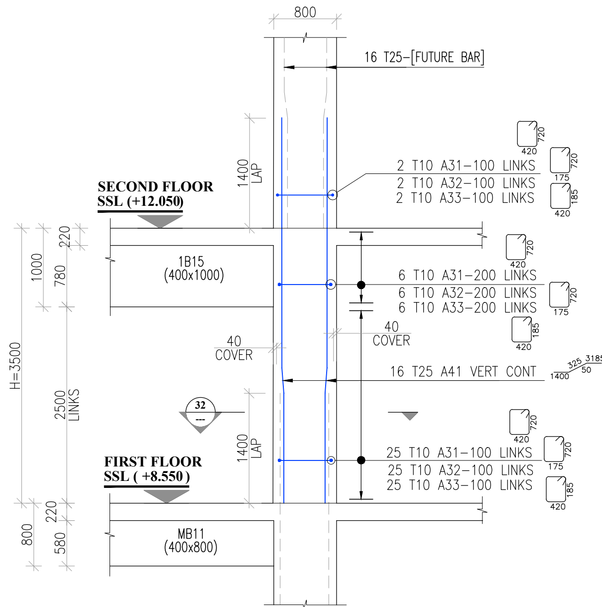
DETAIL-32-C4 (500x800) - 1 No. SCALE 1:50
