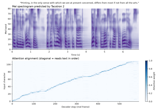
Figure: predicted mel spectrogram (top) and attention alignment (bottom) for a 111-character test sentence.
