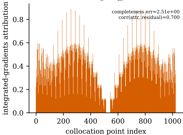
helmholtz_k4 (q_serial)
