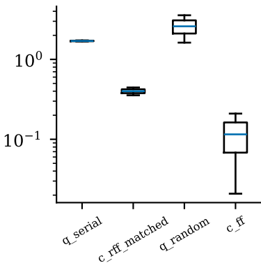
helmholtz_k4
