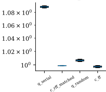
helmholtz_k10
