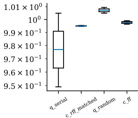
helmholtz_k20
