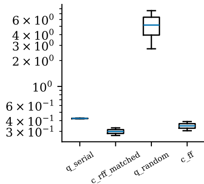
helmholtz_k10
