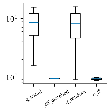
helmholtz_k4
