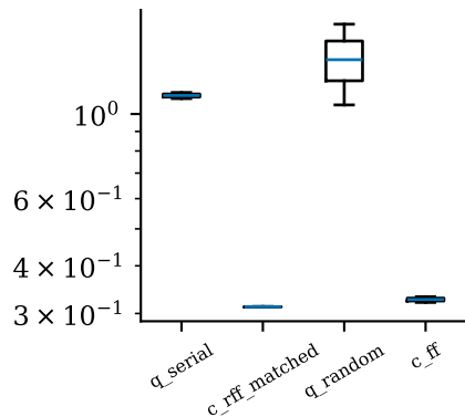
helmholtz_k20
