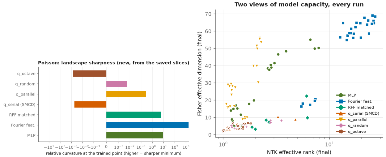
Figure 25: Left: curvature of the loss landscape at the trained point (Poisson). Right: NTK effective rank against Fisher effective dimension, every run.
