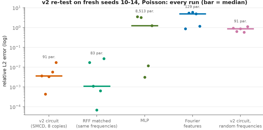
Figure 15: The pre-registered v2 re-test on Poisson: every run on fresh seeds 10–14.
