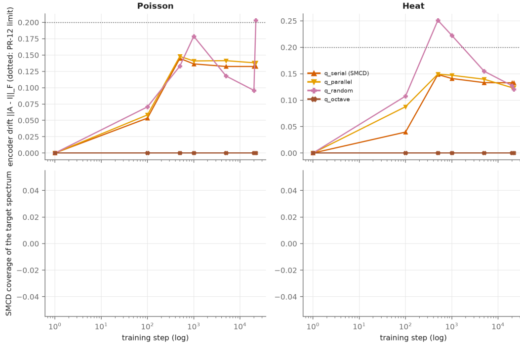
Figure 26: Quantum families: encoder drift \|A - I\|_F (dotted: PR-12's limit 0.2) and SMCD coverage of the target spectrum over training.
