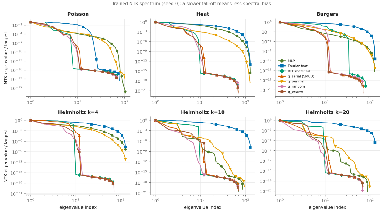
Figure 22: Trained NTK spectra (seed 0), normalised by the largest eigenvalue.
