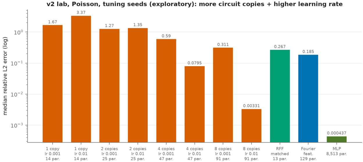
Figure 14: The v2 lab on Poisson, tuning seeds 0–2 (exploratory): median error of each quantum configuration and of the best learning rate for each classical model.
