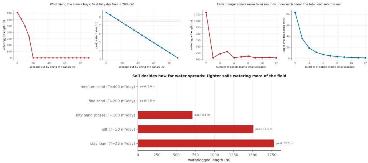
Figure 28: Groundwater scenarios from the exact solution: lining the canals, canal spacing at the same total seepage, and soil type.
