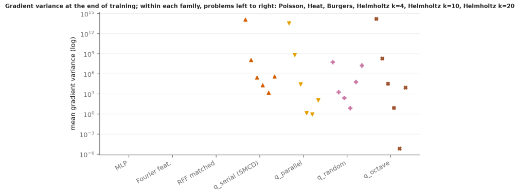
Figure 27: Mean gradient variance at the end of training, per family and problem.
