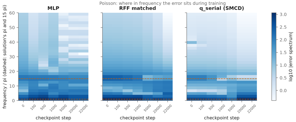
Figure 20: Poisson: magnitude of the error spectrum at each checkpoint (seed 0), with the solution's two frequencies \pi and 15\pi dashed. q_serial removes the 15\pi error early and later loses the \pi component.
