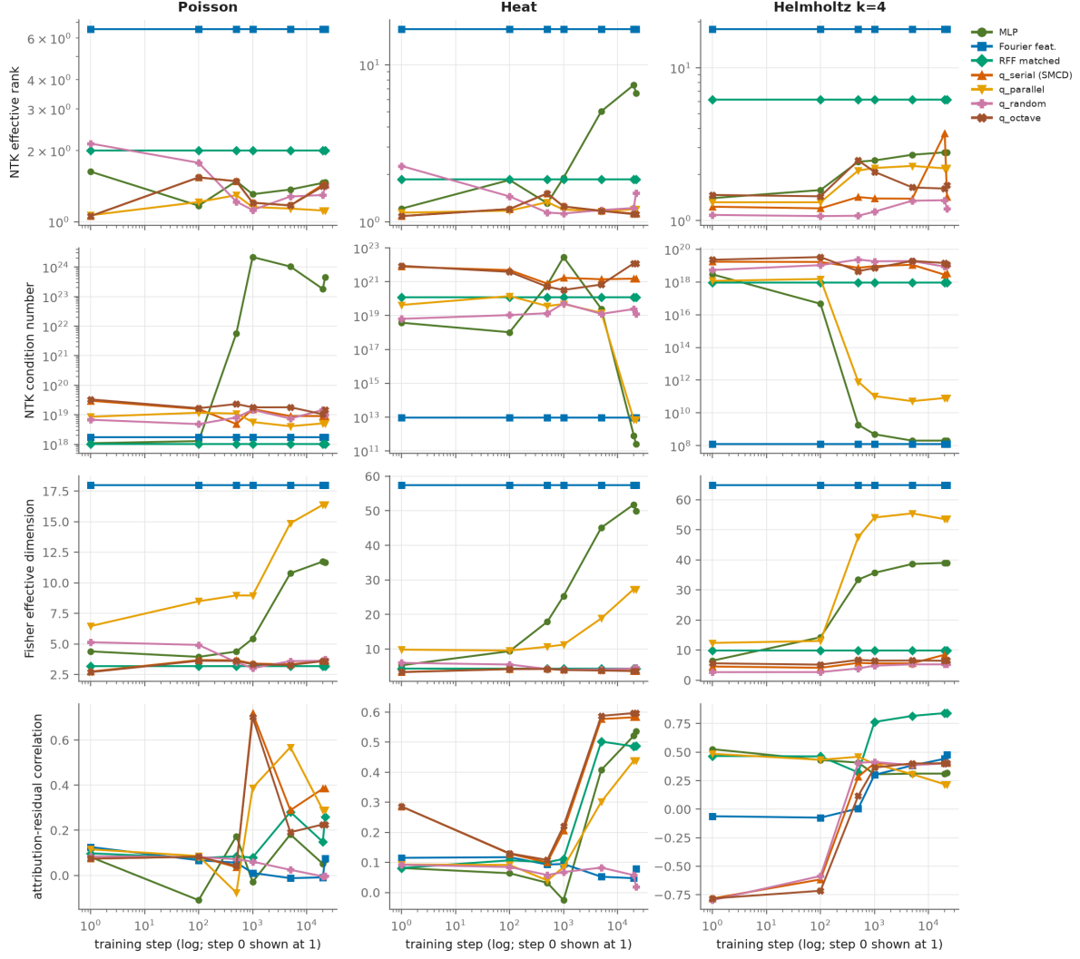
Figure 23: NTK effective rank and condition number, Fisher effective dimension and the correlation of attributions with the residual, over training (median over seeds).
