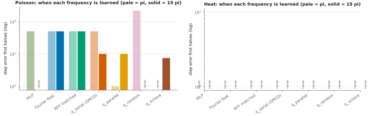
Figure 21: Step at which the error at each solution frequency first halves (median over seeds; pale: \pi , solid: 15\pi ). Left: Poisson; right: heat.
