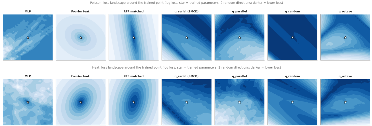
Figure 24: Loss landscape on two random directions around the trained parameters (star), Poisson (top) and heat (bottom); darker is lower loss.
