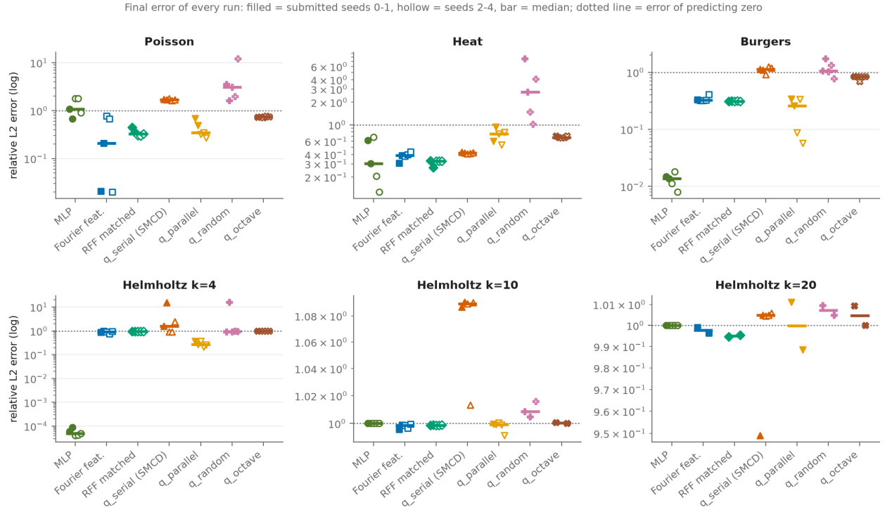
Figure 16: Final relative L^2 error of every core-matrix run at the pre-registered five seeds. Filled: seeds 0–1 (submitted); hollow: seeds 2–4 (post-submission); bar: median; dotted: the error of predicting zero.
