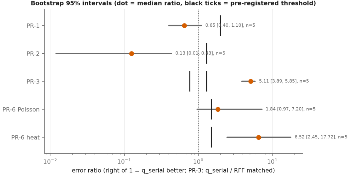
Figure 7: Bootstrap 95% intervals of the pre-registered error ratios (5 paired seeds, 5,000 resamples). Right of 1 means q_{\text{serial}} is better; for PR-3 the ratio is q_{\text{serial}}/c_{\text{rff\_matched}} and must lie between the two ticks.
