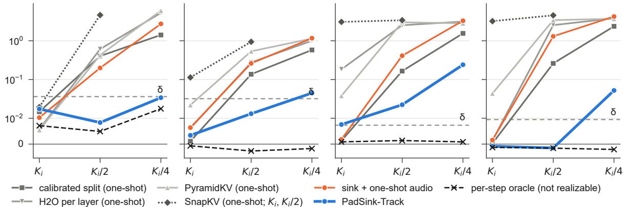
(a) Whisper-medium, Uzbek
