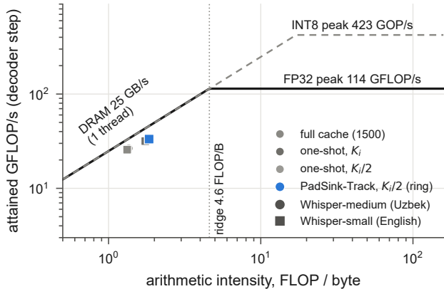
(a) Roofline, 1 thread
