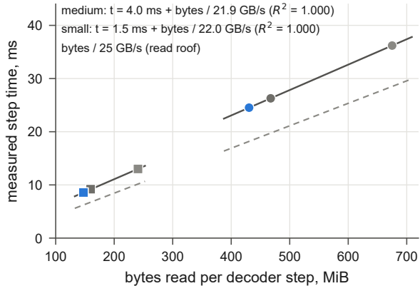
(b) Step time is linear in the bytes read
