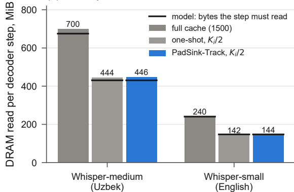
(a) Memory-controller counters vs. model
