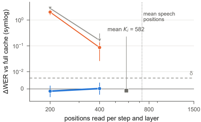
(a) Whisper-small, English, \geq 10 s ( n = 80 )
