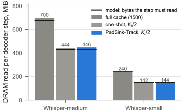
(a) Memory-controller counters vs. model
