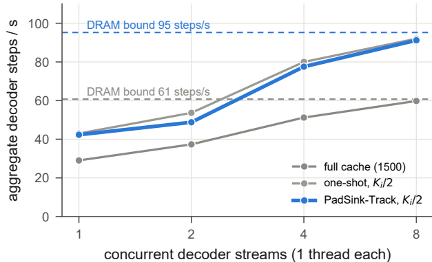
(b) Throughput of N streams sharing DRAM (medium)
