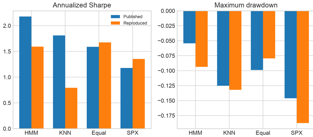
Figure 1: Published targets and independently reproduced outcomes. The gap is not a confidence interval; it is a discrepancy between two implementations whose specifications are not identical because the target implementation is undisclosed.
