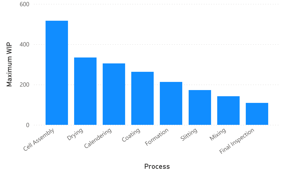
Max WIP by Process
