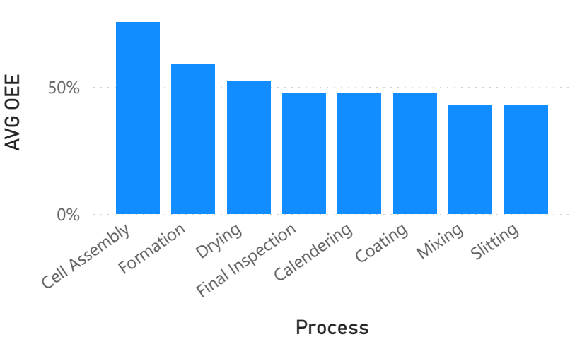
OEE BY PROCESS
