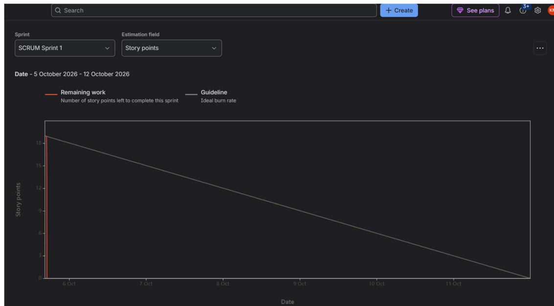
Figure X: Sprint 1 Burndown Chart
