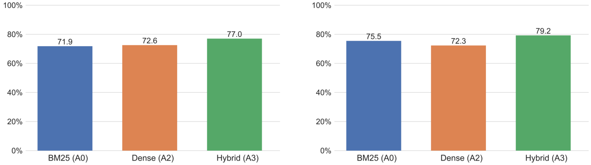
Figure 2: Accuracy on non-OOD queries (pooled; n = 135 and 159 , including the 25 canonical controls) for BM25, dense-only, and hybrid retrieval. Left: v0.1. Right: v0.2.
