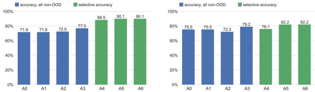
Figure 6: Ablation A0–A6. A0–A3: accuracy on all non-OOD queries (pooled). A4–A6: selective accuracy on the queries each configuration answers (mean over folds), at reduced coverage, so not directly comparable to A0–A3. Left: v0.1. Right: v0.2.
