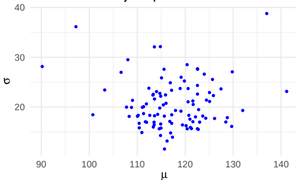
Draws from the joint posterior distribution
