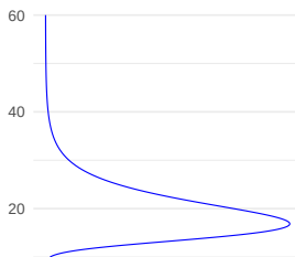
Marginal of sigma
