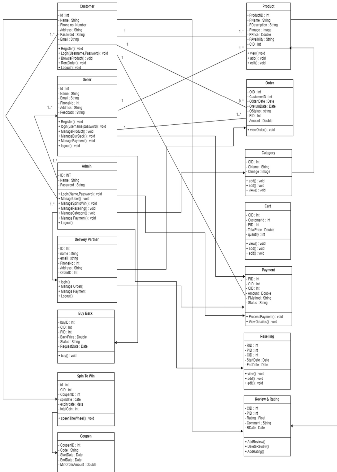
Figure 9 Class Diagram
