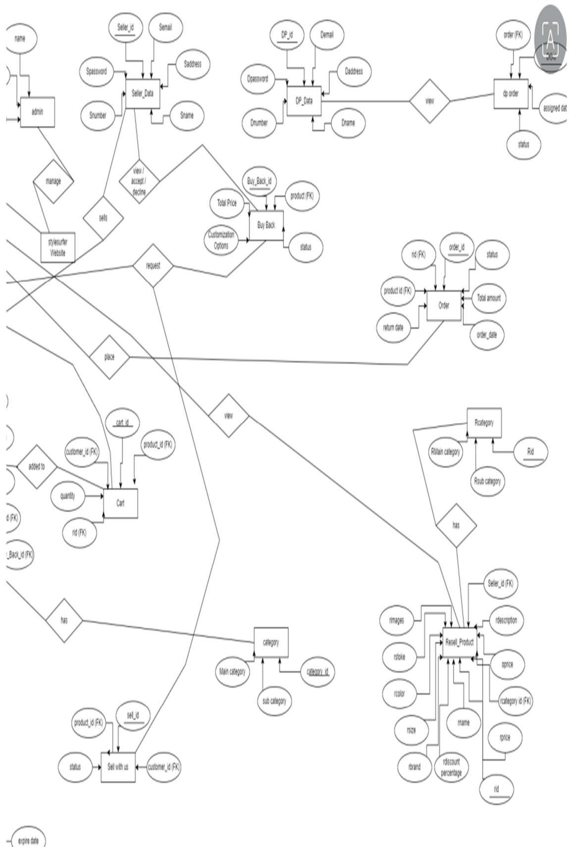
Figure 2 E.R. Diagram
