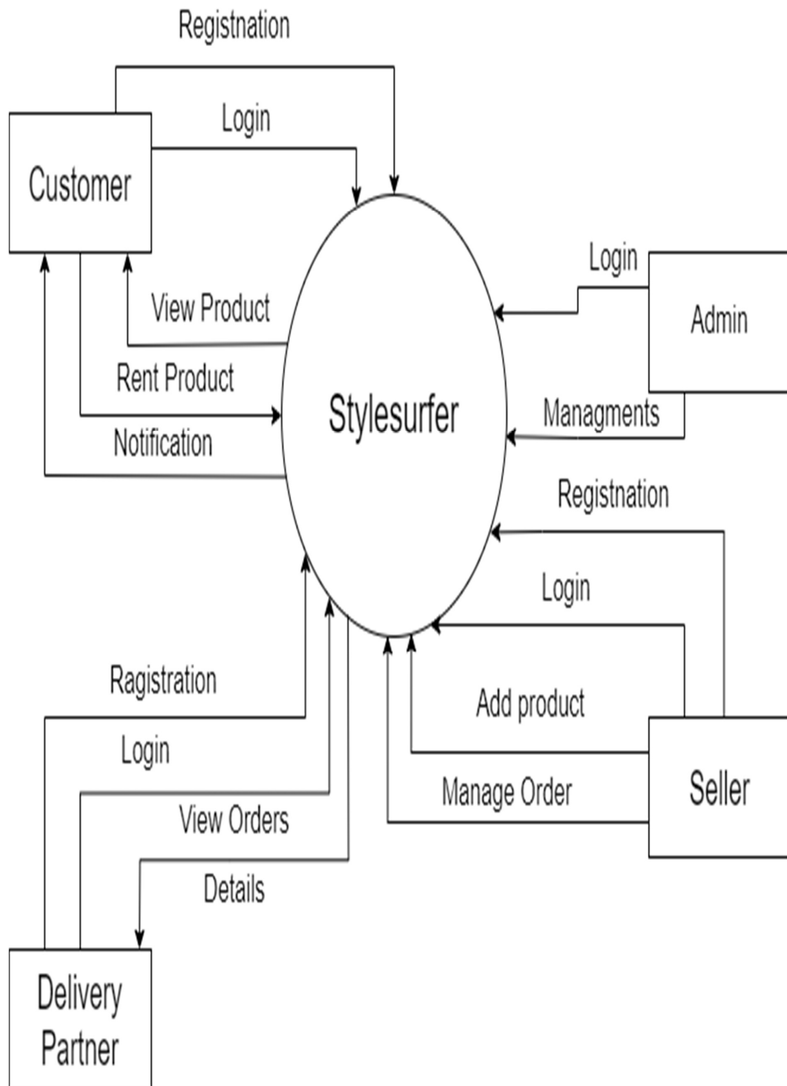
Figure 5 DFD (Level 0)
