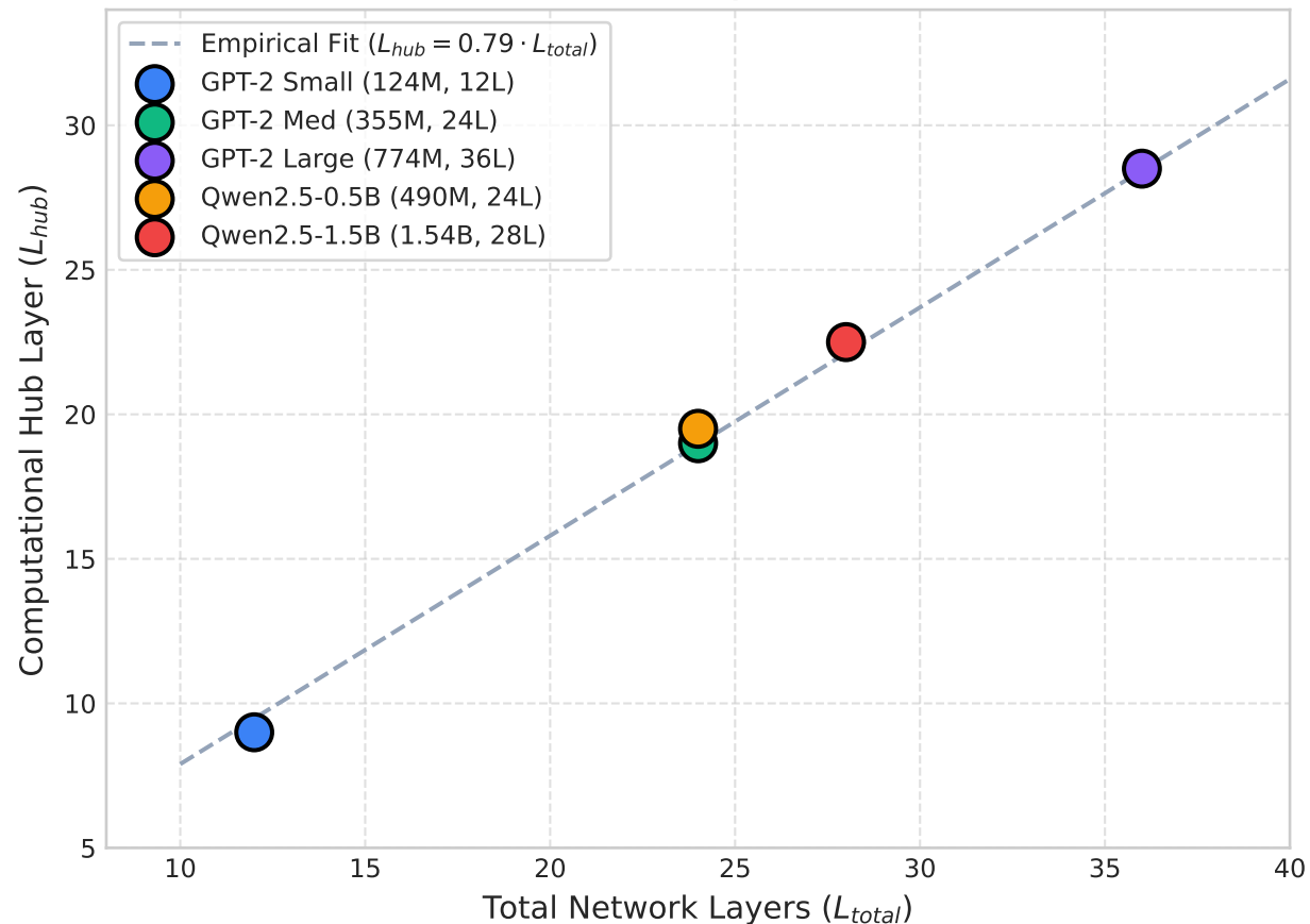
Computational Hub Layer vs. Total Depth
