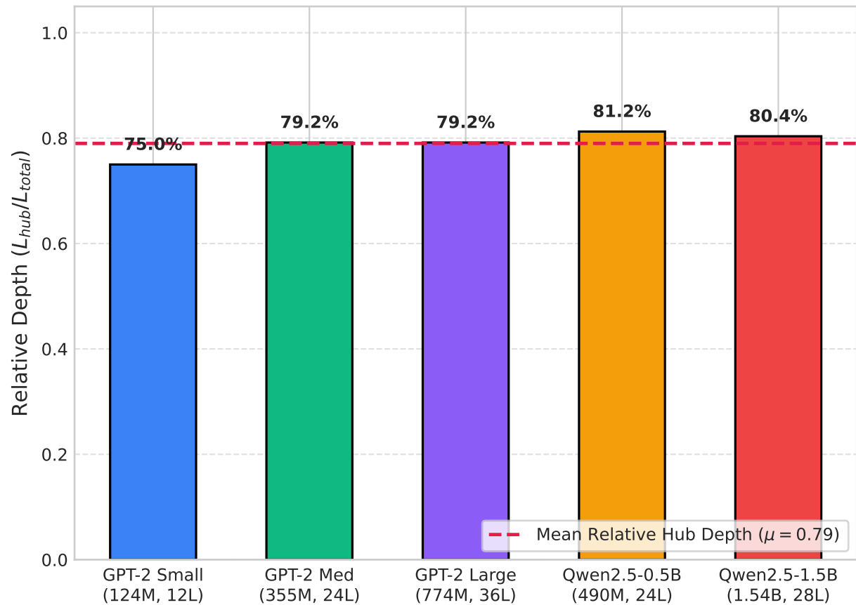
Universal Relative Depth Invariance Across Architecture Families
