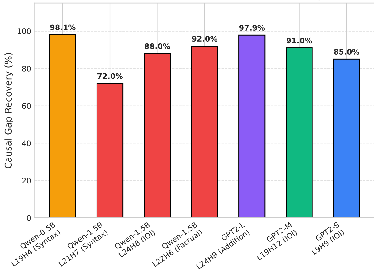
Isolated Single-Head Causal Gap Recovery
