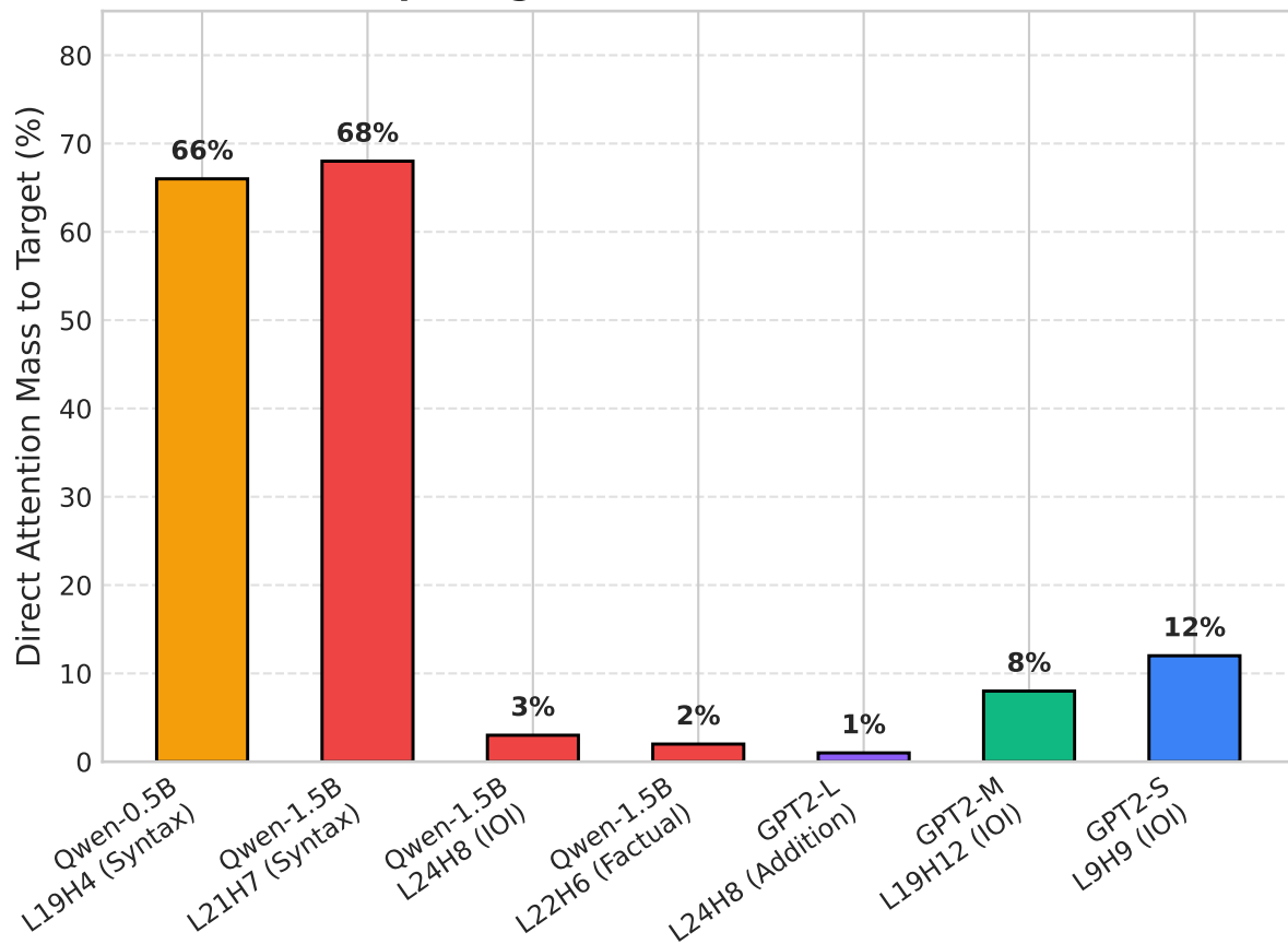
Attention Sharpening: RoPE (Qwen) vs. Absolute PE (GPT-2)
