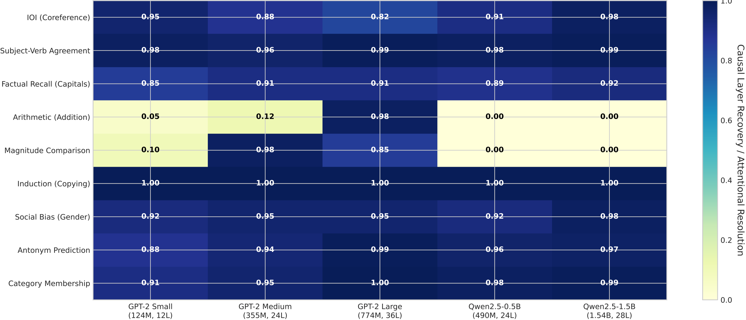
Cross-Model Cognitive Capability & Circuit Attribution Map
