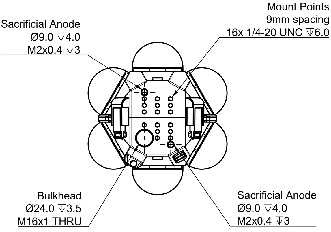
Bottom View
