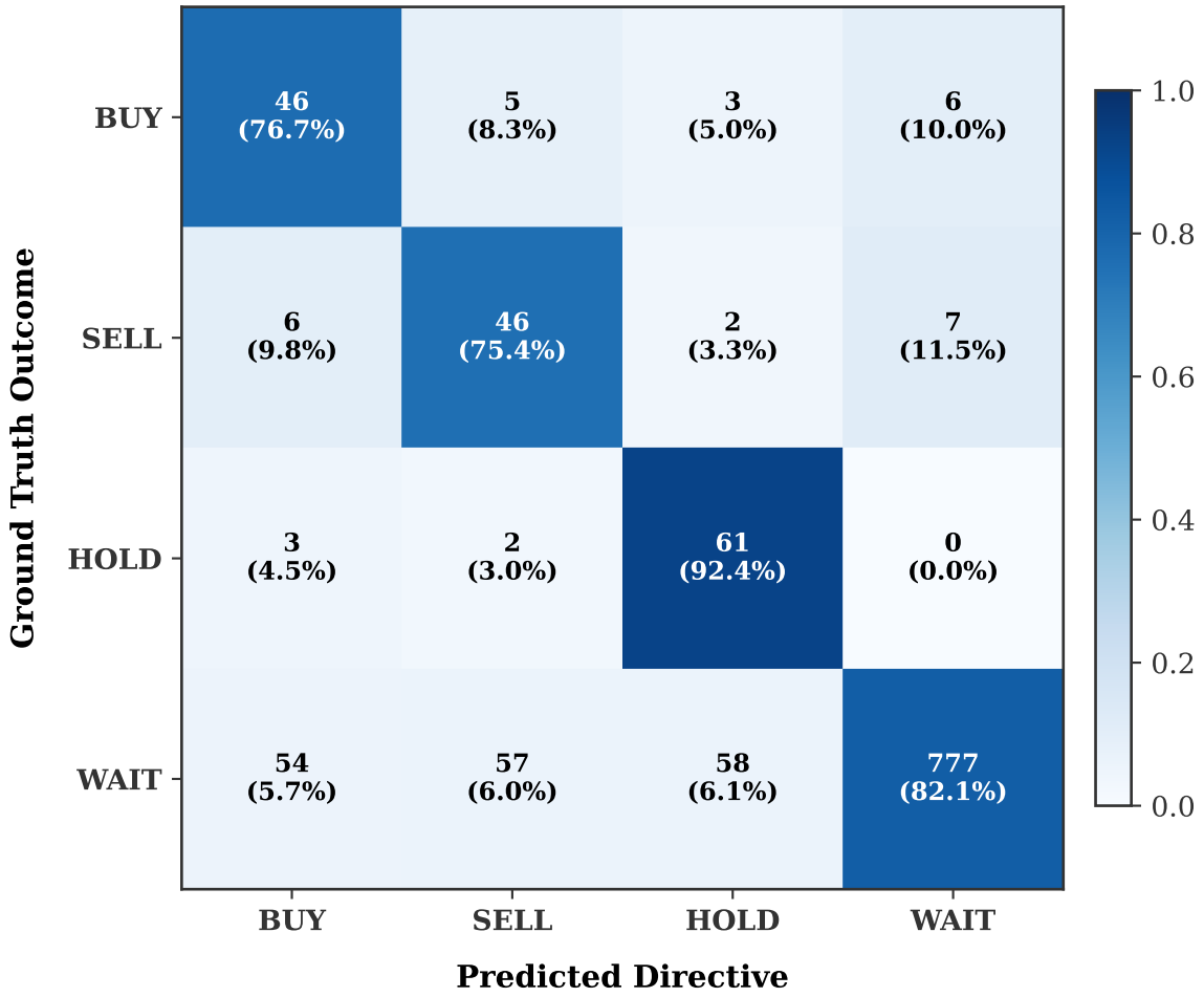
Figure 5.7(a): Decision Engine Normalized Confusion Matrix
