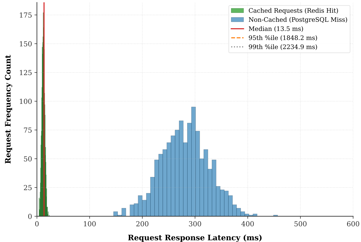
Figure 5.9(a): FastAPI Request Latency Distribution
