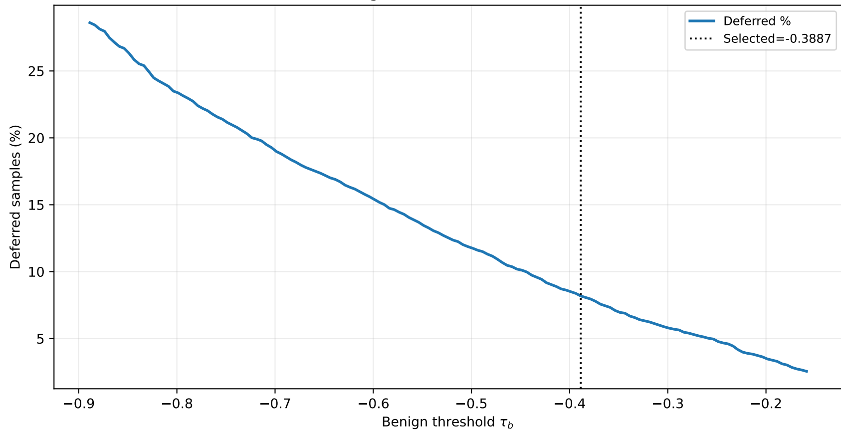
Deferred % vs benign threshold (malware threshold fixed)
