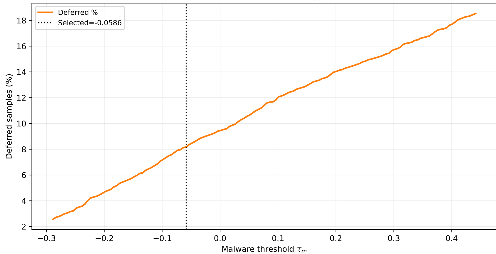
Deferred % vs malware threshold (benign threshold fixed)
