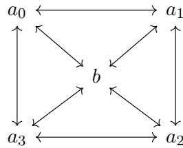
Figure 2: Splitting the closed path p into triangles.
