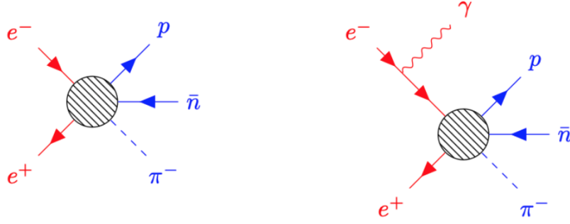
Figure 5.2: Feynman diagram of the channel of interest. Phokhara handles the initial hard photon emission (red), while EvtGen simulates the decay to final-state particles (blue).
