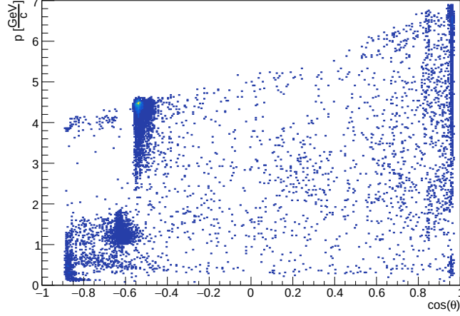
Figure 7.2: 2D \cos(\theta) vs momentum distribution in data, NO ISR case.
