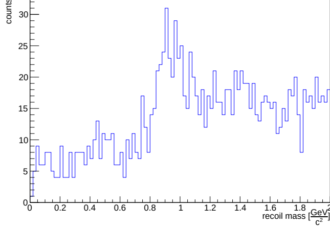
Figure 7.3: Recoil mass distribution in data, NO ISR case. Cut -0.45 < \cos(\theta) < 0.85 applied, on the reconstructed protons.
