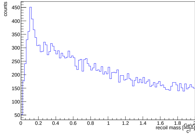
Figure 7.1: Recoil mass distribution in data, NO ISR case.
