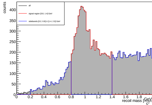
Figure 6.15: Recoil mass distribution (black), with the signal region (red) and the sidebands regions (blue), in the q\bar{q} Monte Carlo cocktail. NO ISR case.
