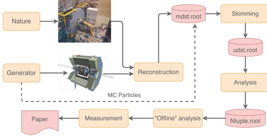
Figure 3.5: A scheme of the Belle II Data Model, starting from the nature processes information to the final results. Monte Carlo truth information bypasses reconstruction, since the information is directly picked at generator level.
