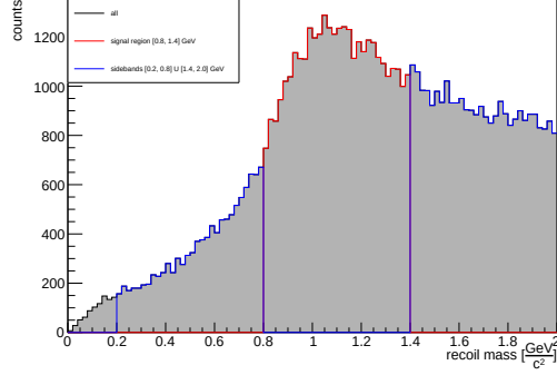
Figure 6.20: Recoil mass distribution (black), with the signal region (red) and the sidebands regions (blue), in the q\bar{q} Monte Carlo cocktail. ISR case.
