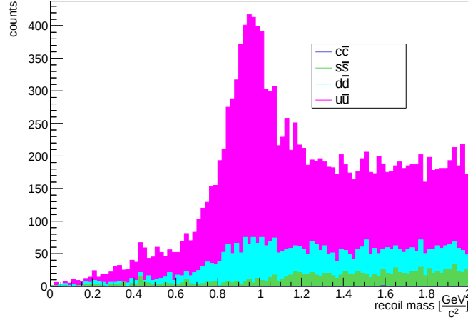
Figure 6.12: p, \pi^- recoil mass distribution in q\bar{q} Monte Carlo cocktail, displaying each stacked q\bar{q} component contribution, NO ISR case. (pink) u\bar{u} component; (light blue) d\bar{d} component; (green) s\bar{s} component; (blue) c\bar{c} component.
