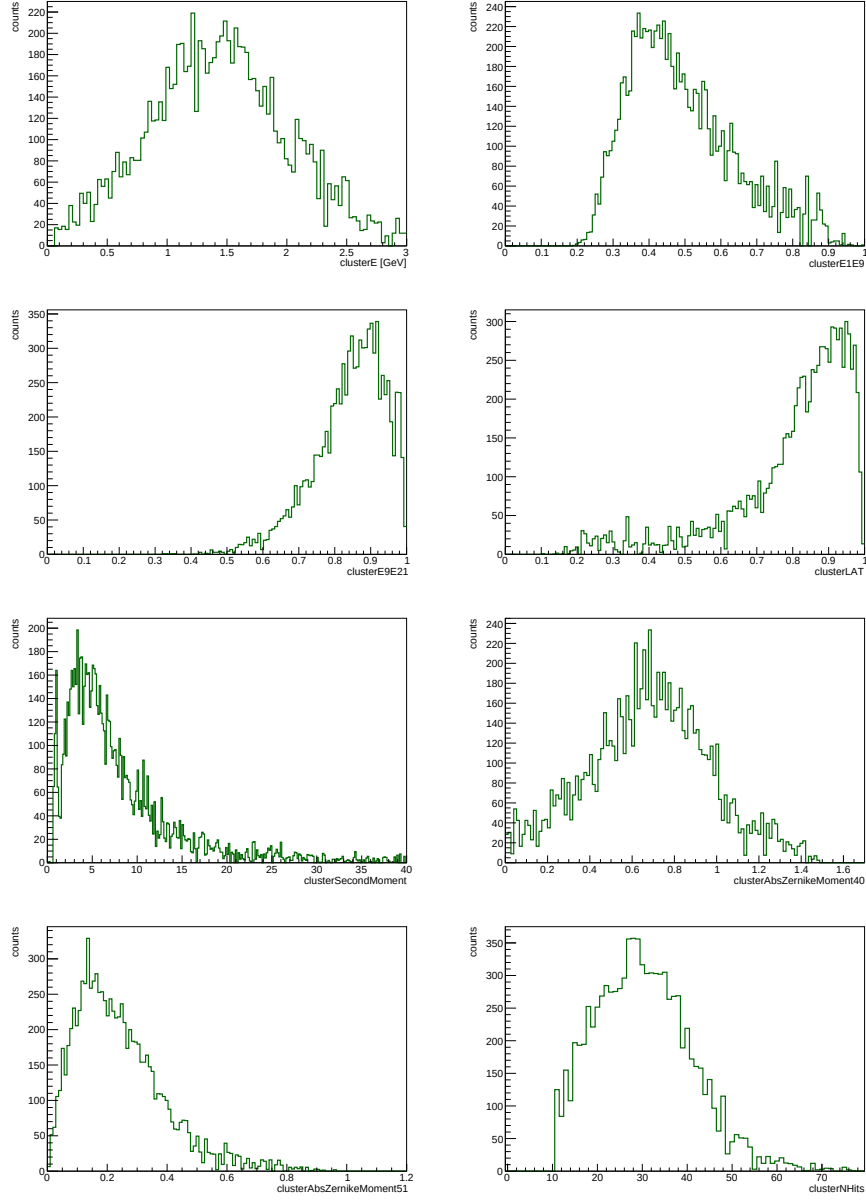
Figure 6.22: Reconstructed cluster variables for \bar{n} candidates after the application of the sidebands subtraction, in ISR case. \bar{q} cocktail.
