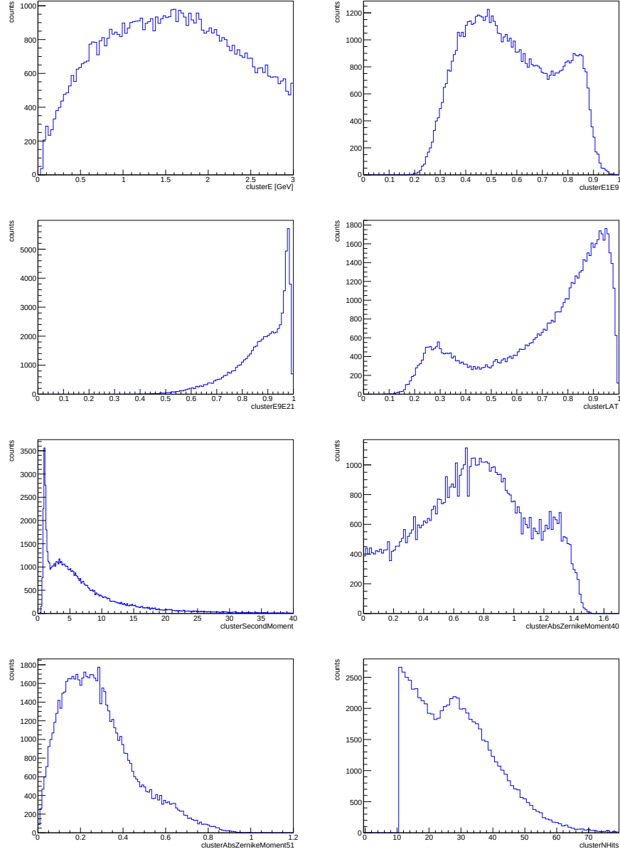
Figure 9.5: Reconstructed cluster variables distribution for \bar{n} candidates in the for the recoil mass region [0, 2] GeV, in ISR case. q\bar{q} cocktail
