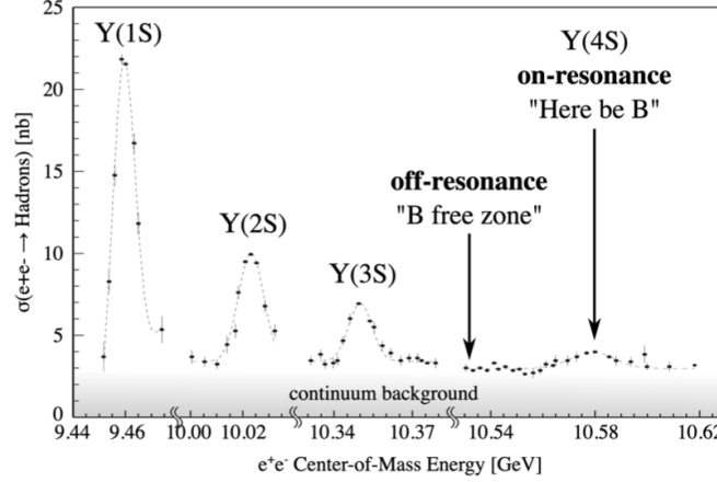
Figure 6.4: Cross section of e^+e^- \rightarrow \text{Hadrons} , in \Upsilon resonances energy region [5]. \Upsilon(1S) resonance is very narrow, while \Upsilon(4S) one is broader and lower
