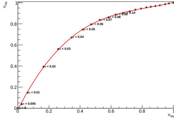
Figure 6.13: Receiver Operating Characteristic (ROC) curve constructed from the signal efficiency ( \epsilon_{sig} ) and the Background Efficiency ( \epsilon_{bkg} ) for the u\bar{u} Monte Carlo cocktail. where each point corresponds to a different cut value on the \alpha angle. For clarity, the labels are shown only for \alpha < 0.10 rad.
