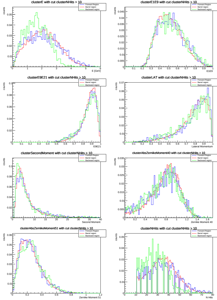
Figure 5.32: Comparison of reconstructed cluster variables for all \bar{n} candidates in different ECL regions. The distributions are normalized to unit value
