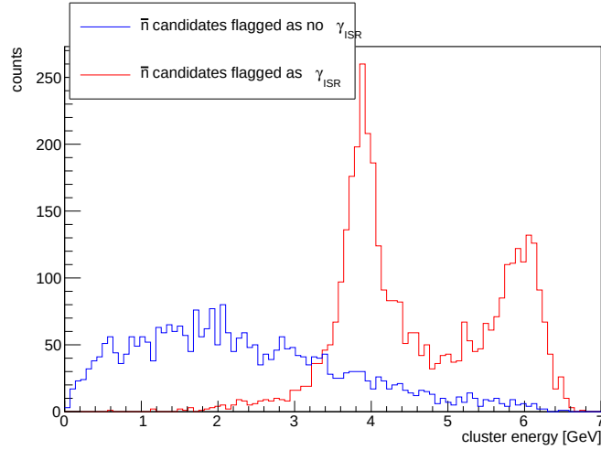
Figure 6.6: Cluster energy distribution of \bar{n} candidates, divided by the Monte Carlo ISR flag ( \text{mcISR} ). If \text{mcISR} = 0 , the reconstructed particle is not an ISR photon. If \text{mcISR} = 1 , the reconstructed particle is an ISR photon. Of course this is a level-generator information.
